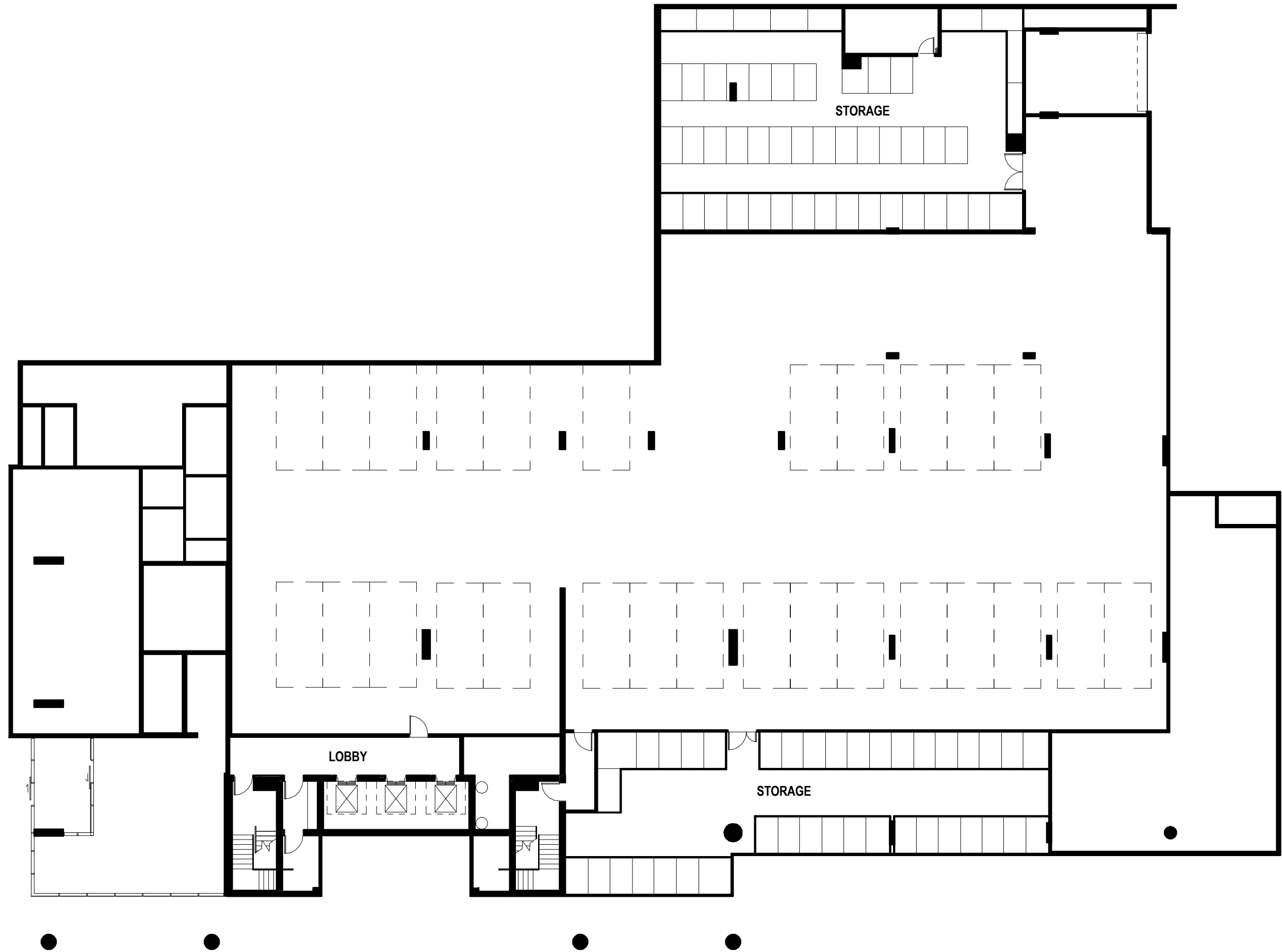
Contract Plan - Level 01
